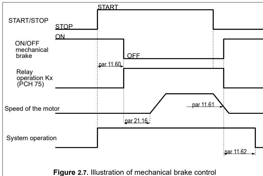
Figure 2.7. Illustration of mechanical brake control
